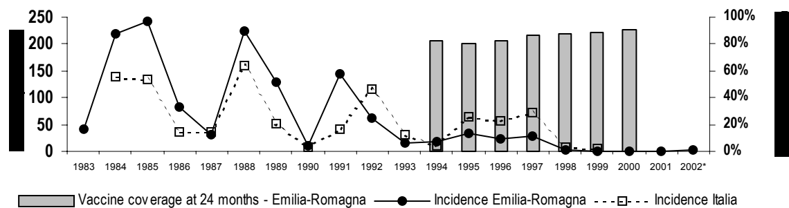
Figure 1 – Measles incidence per 100,000 in Emilia-Romagna and Italy, 1983-2002* and vaccine coverage between 24 and 36 months in Emilia-Romagna, 1994-2000
